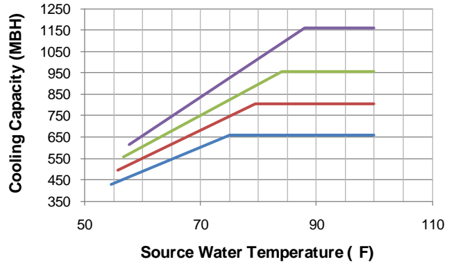
HPW60M Cooling Capacity vs. Source Water Temperature
