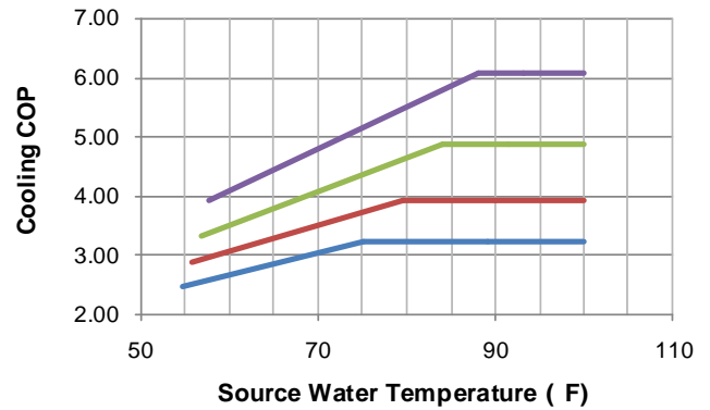
HPW60 Cooling COP vs. Source Water Temperature
