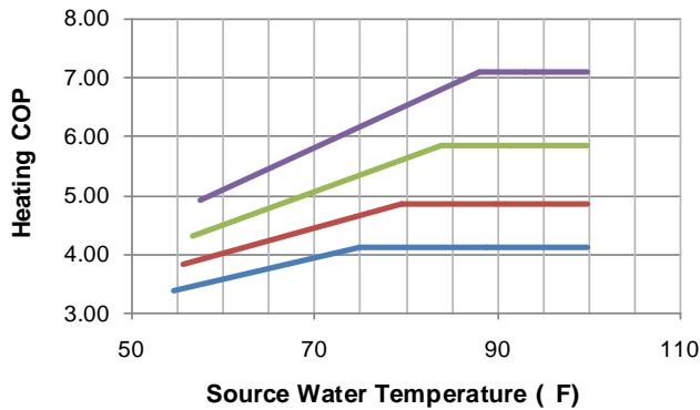
HPW60 Heating COP vs. Source Water Temperature
