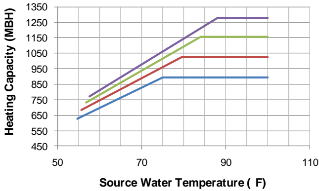
HPW60M Heating Capacity vs. Source Water Temperature
