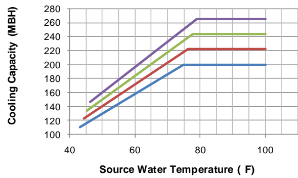
HPW15 Cooling Capacity vs. Source Water Temperature
