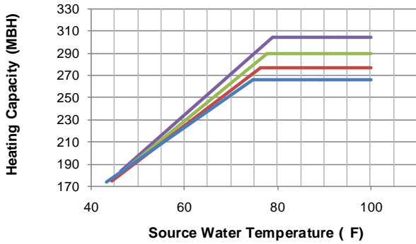
HPW15 Heating Capacity vs. Source Water Temperature
