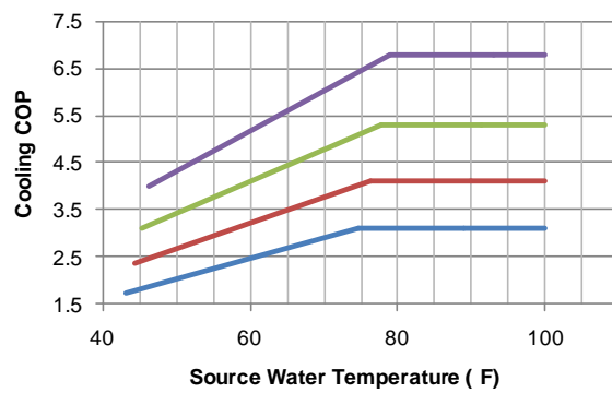
HPW15 Cooling COP vs. Source Water Temperature
