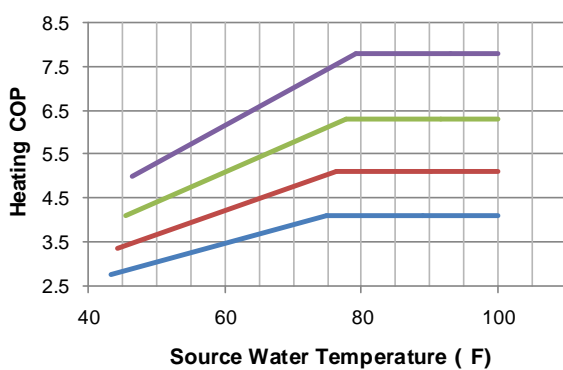
HPW15 Heating COP vs. Source Water Temperature
