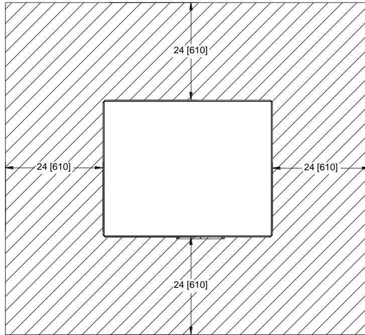
SERVICE CLEARANCE
