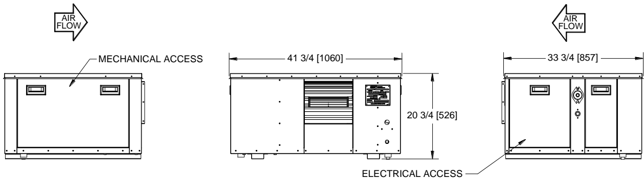
SERVICE CLEARANCE
